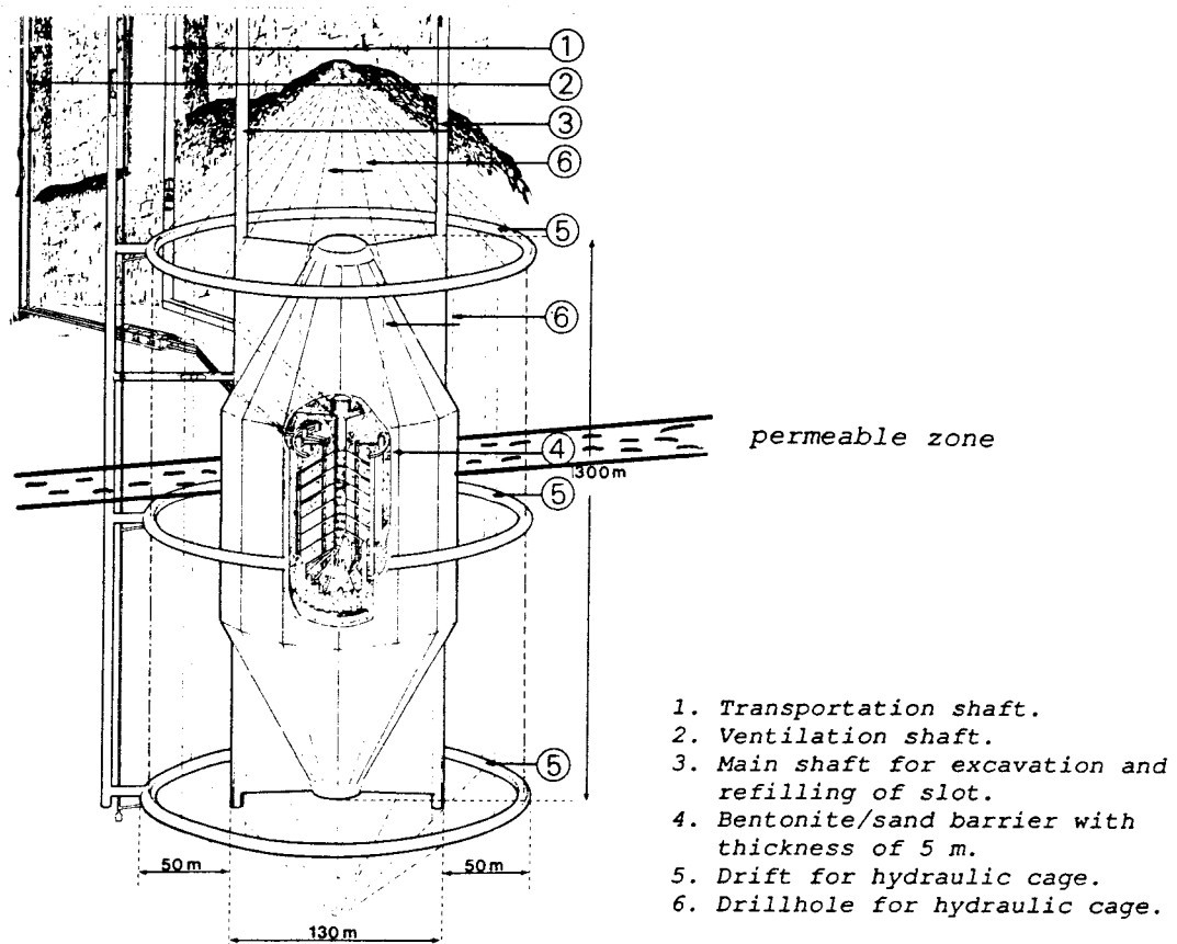
Figure 14-1. Permeable zone intersected by a WPC.
